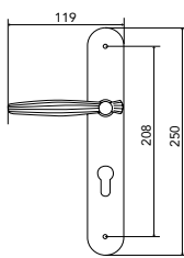
Door handles on plates
