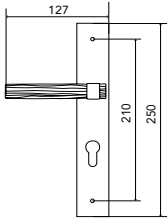
Door handles on plates
