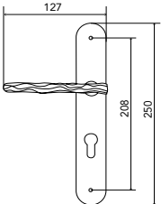
Door handles on plates
