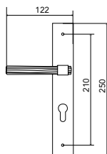
Door handles on plates
