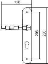
Door handles on plates
