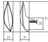
LEAF 62 Knobs
