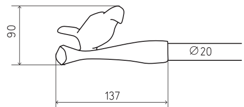
EMBOUT PLUME 20
