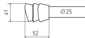
EMBOUT ORBE 25
